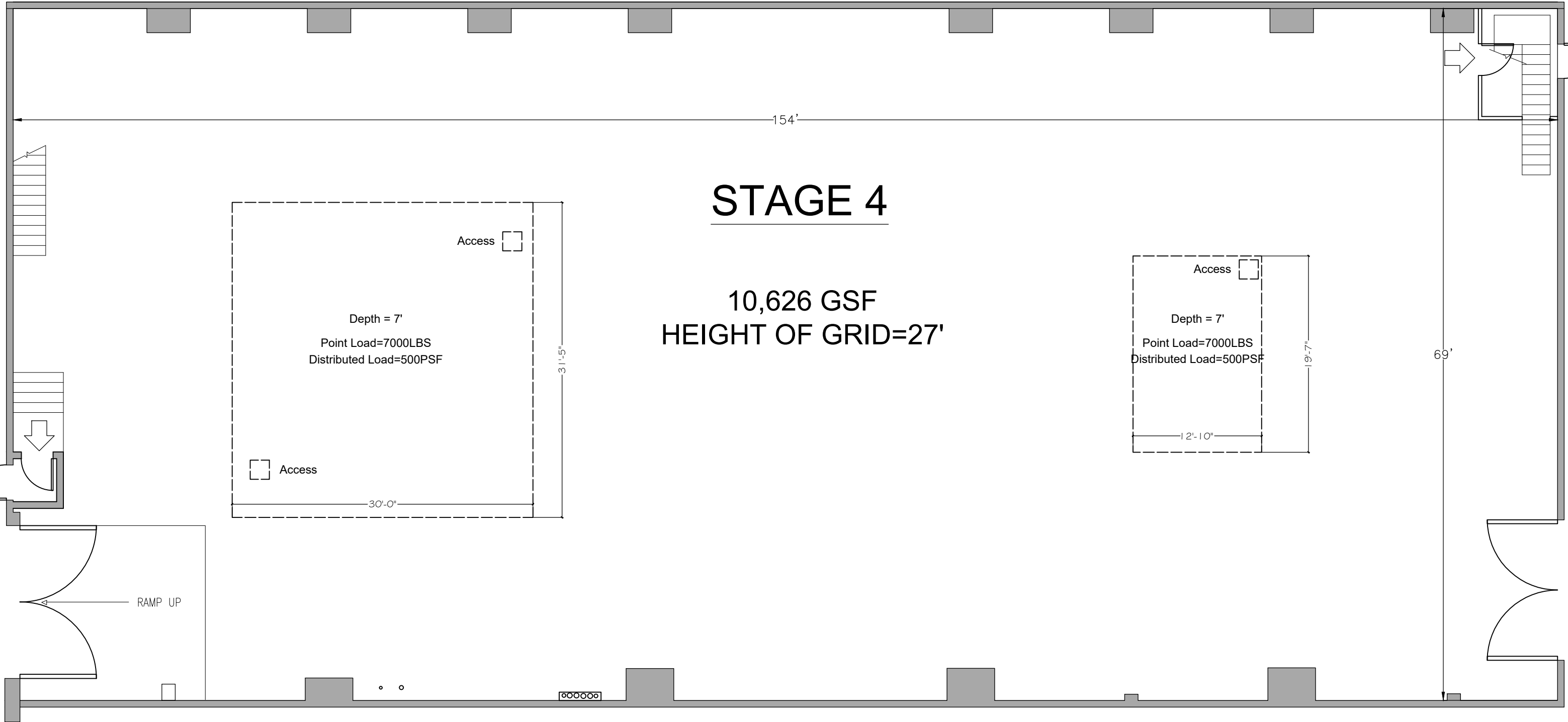
STAGE FLOOR PLAN
