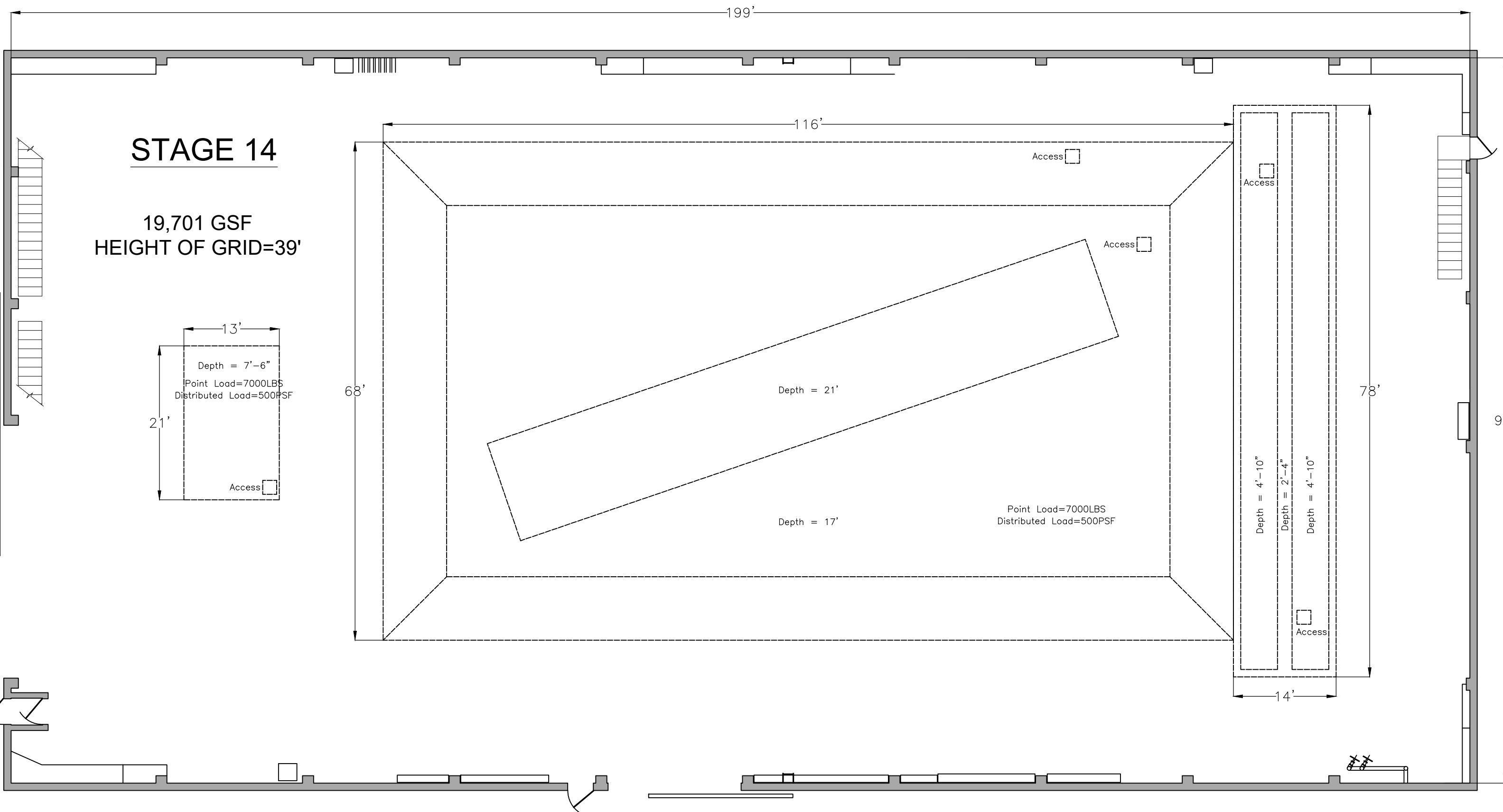
STAGE FLOOR PLAN
